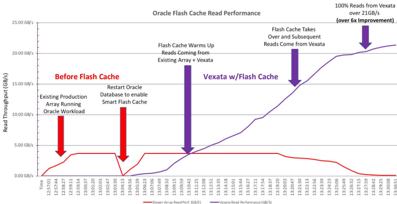
Figure 2: Oracle RAC Read Throughput Performance with Smart Flash Cache and Vexata VX-100F
